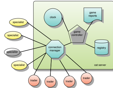
Figure 1: The topology of a CAT game.
